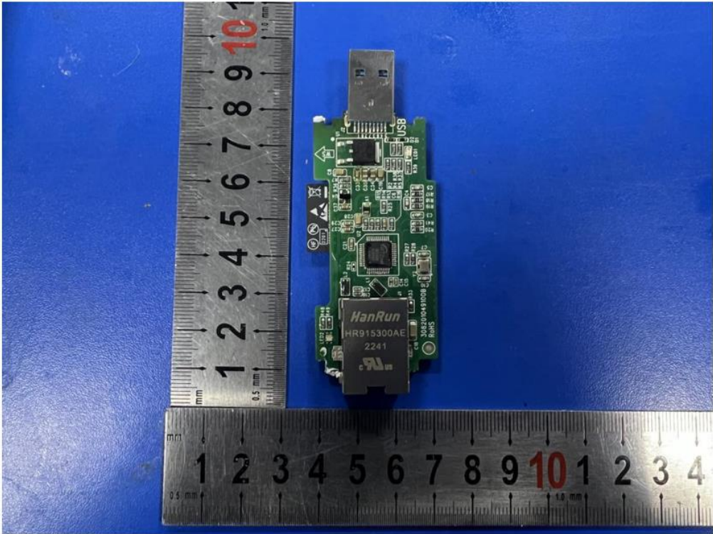
Fig.4 PCB top view
